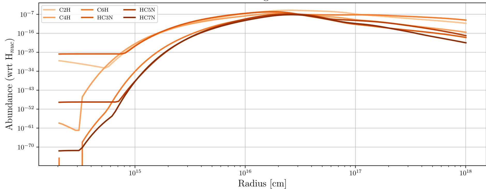
Particle 0 - Daughter Molecules
